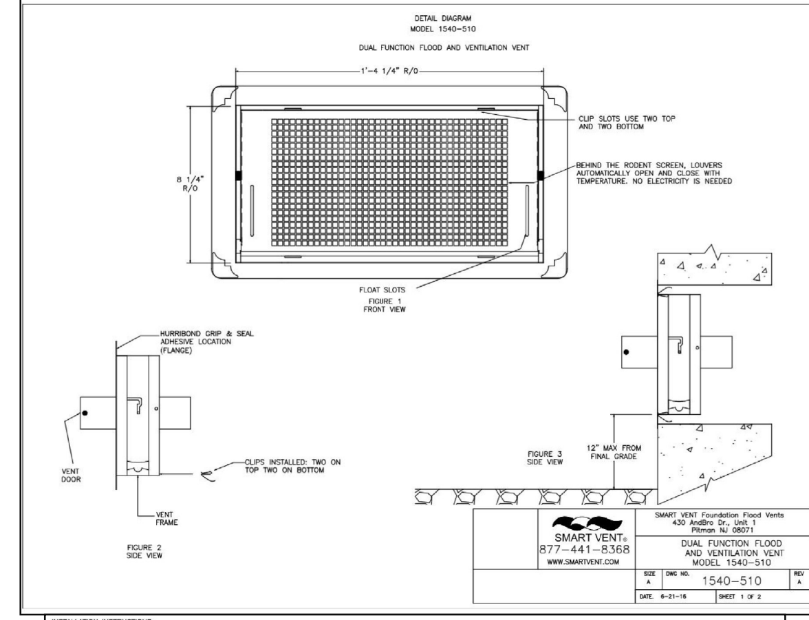
FLOOD VENT DETAILS
